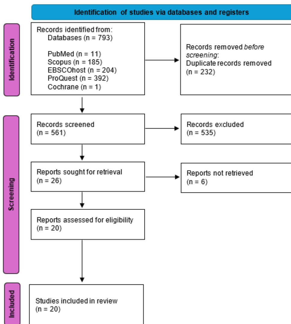
Fig. 1: PRISMA flowchart
