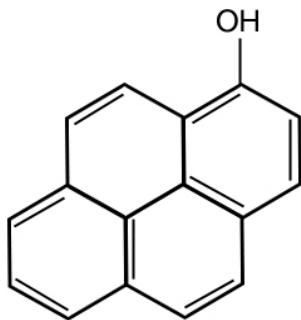
Fig. 1: Chemical structure of 1-hydroxypyrene
