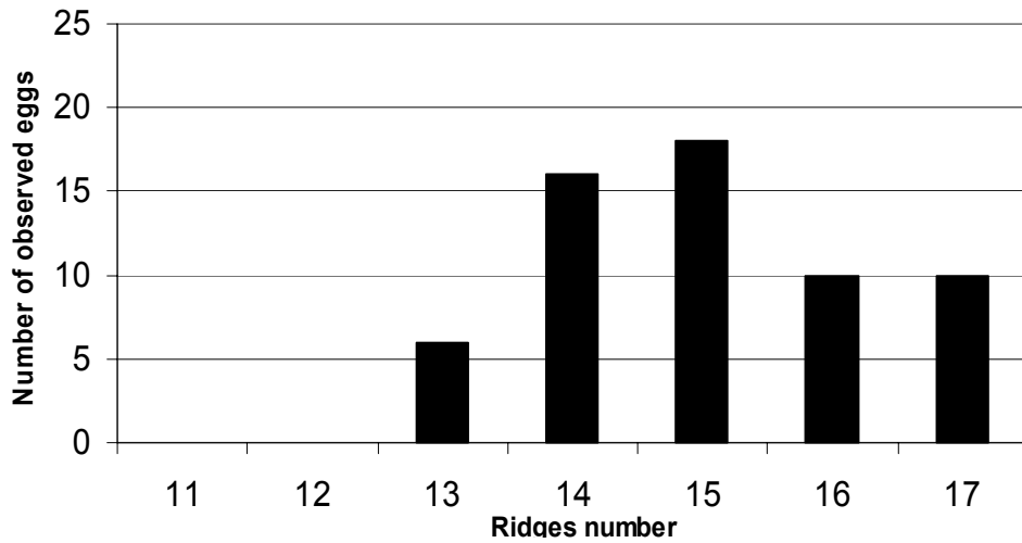
Fig. 3: Egg float ridges distribution of each population within Kazerun population of An. stephensi .
