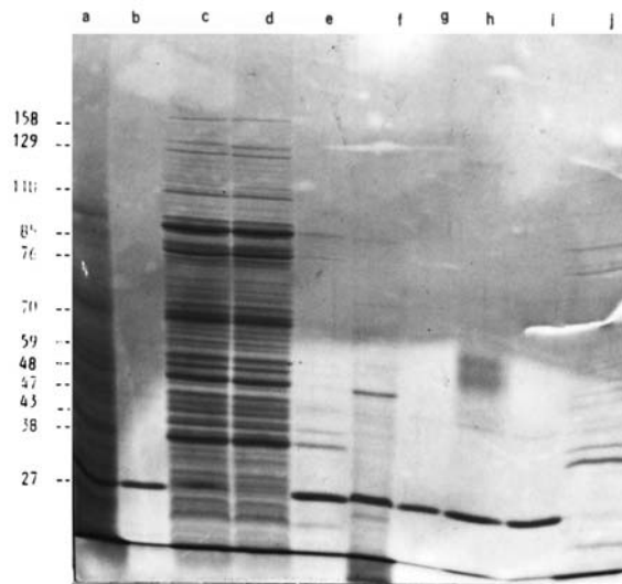
Fig. 1 Comparison between different fraction of S. aureus Bate conventionally prepared PG, lysostaphin, crude antigen treated with lysostaphin, non- treated crude with lysostaphin, modified PG, TA, LTA and PA are show in tracks a to h. Lysostaphin and crude antigen after three minutes sonication are shown in tracks i and j. The molecular weights of some polypeptide bands are shown by the number ( \times 10^3 ) on the vertical axis. Electrophoresis of the samples were done in 10% polyacrylamide gels.
