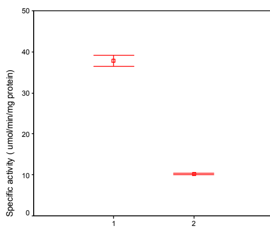
Fig. 3: GSTs specific activity of purified solutions from sheep liver tissue: 1 and Protoscoleces: 2
