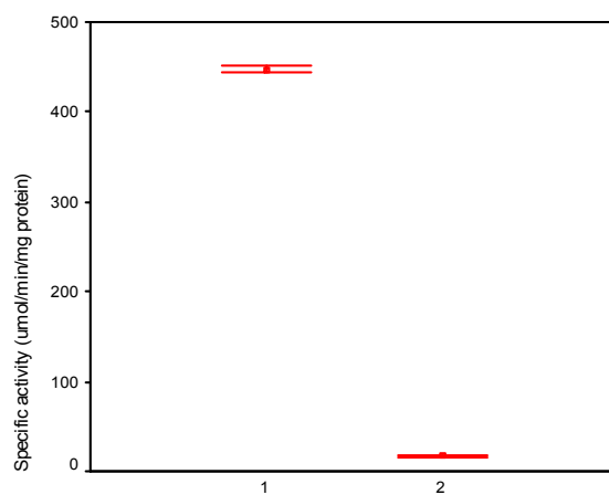
Fig. 2: GST specific activity of extract solutions from sheep liver tissue: 1 and protoscoleces: 2
