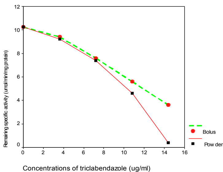
Fig. 7: GST remaining specific activity based on triclabendazole concentration in the purified solution of protoscolexes.
