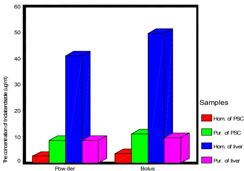
Fig. 8: Inhibition concentrations of 50% of GSTs specific activity (IC 50 ) of protoscolexes and sheep liver tissue by triclabendazole (powder & bolus).
