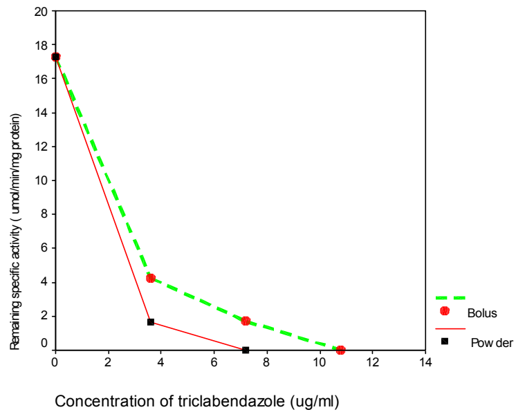
Fig. 6: GST remaining specific activity based on triclabendazole concentration in the extract solution of protoscolecis.
